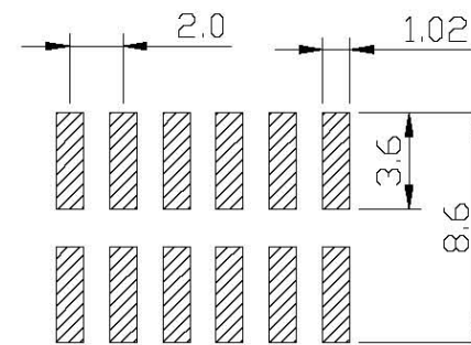
Recommended P.C.B Hole Layout
